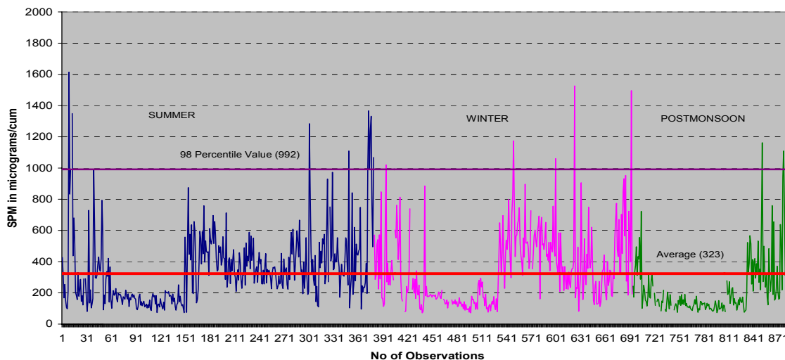
SPM Variation in AAQ_Western Zone
