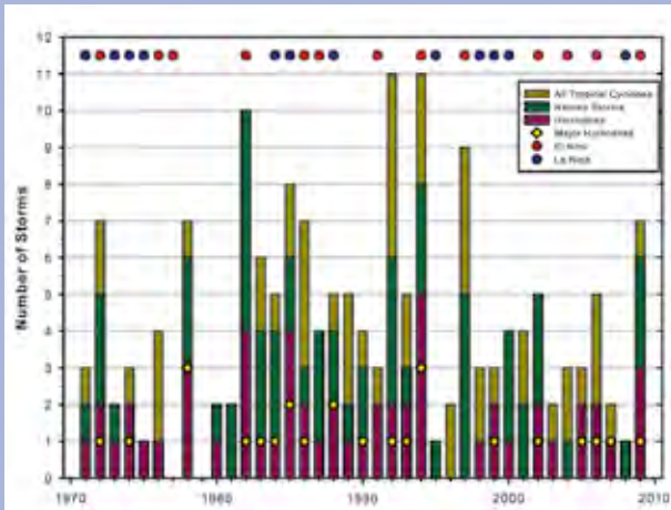
FIG. 4.37. Annual TC activity in the CNP, 1971–2009, with seasonal totals of: TCs including TDs (brown), NSs (green), Hs (purple), and MHs (yellow diamonds). Circles at top denote the ENSO phase (El Niño: red, La Niña: blue) for each TC season.
