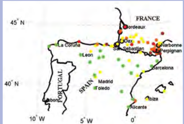
FIG. 7.36. Maximum wind gusts recorded in Spain and southern France (on either 23 or 24 January 2009). Green (100–120 km hr -1 ), yellow (120–140 km hr -1 ), orange (140–160 km hr -1 ), red (160–180 km hr -1 ), and brown (180–200 km hr -1 ). Stations which set new wind gust records are highlighted with a solid circle around the color circle.
