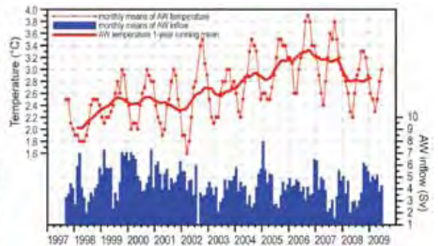
FIG. 5.9. Mean temperature of Atlantic water (AW, defined with TAW > 1°C) and the AW volume inflow in the West Spitsbergen Current, northern Fram Strait measured by the array of moorings at 78°50'N.
