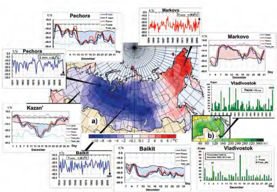
FIG. 7.39. Weather conditions in December 2009 (a) Air temperature anomalies. Insets show the series of mean monthly and mean daily air temperatures in December 2009 at meteorological stations Pechora, Baikit, Markovo, and Kazan; (b) Percentage of monthly mean precipitation in the southern Far East. Insets show the series of monthly and daily precipitation totals in December 2009 at meteorological station Vladivostok.
