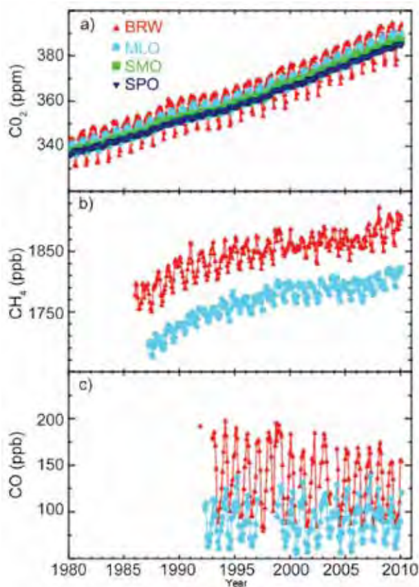
FIG. 2.35. Monthly mean mole fractions determined from NOAA/ESRL Observatories at Barrow, Alaska (BRW); Mauna Loa, Hawaii (MLO); American Samoa (SMO); and South Pole (SPO) for (a) CO 2 , (b) CH 4 , and (c) CO. 2009 results are preliminary. Monthly means are courtesy of Kirk Thoning (CO 2 ), Ed Dlugokencky (CH 4 ), and Paul Novelli (CO), all from NOAA/ESRL. Additional plots can be found at: http://www.esrl.noaa.gov/gmd/ccgg/iadv/ and http://www.esrl.noaa.gov/gmd/Photo_Gallery/GMD_Figures/ccgg_figures/ .
