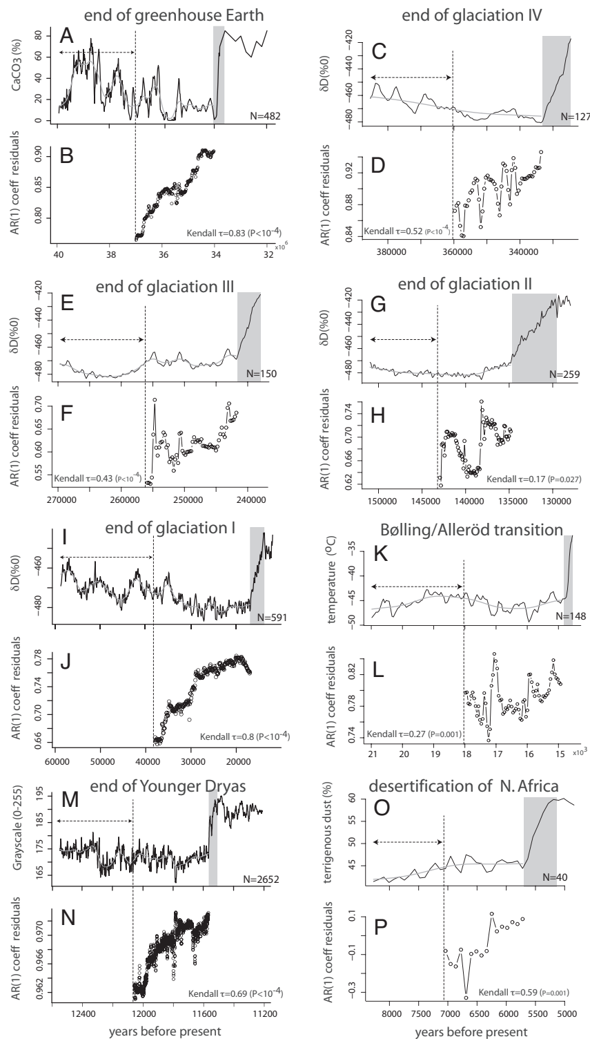
Fig. 1. Eight reconstructed time series of abrupt climate shifts in the past. (A) The end of the greenhouse Earth, (M) the end of the Younger Dryas, (K) the Bolling-Allerod transition, (O) the desertification of North Africa, (I) the end of the last glaciation, and (G, E, and F) the ends of earlier glaciations. In all cases the dynamics of the system slow down before the transition, as revealed by an increasing trend in autocorrelation (B, D, F, H, J, L, N, and P). The gray bands identify transition phases. The arrows mark the width of the moving window used to compute slowness. The smooth gray line through the time series is the Gaussian kernel function used to filter out slow trends. Data in A come from tropical Pacific sediment core records, data in M are from the Cariaco basin sediment, data in K come from the Greenland GISP2 ice core, data in O from the sediment core ODP Hole 658C off the west coast of Africa, and data presented in C, E, G, and I are from the Antarctica Vostok ice core (additional details are in supporting information (SI) Table S1 and Fig. S1 ).
