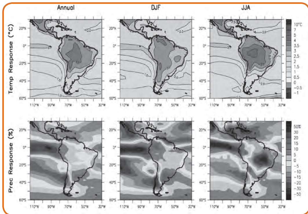
Figure 5. Multi-model simulations of temperature and precipitation changes towards the end of the century compared to historical averages. Left panel – annual mean; middle panel – December to February; right panel – June to August (Ch. 11, IPCC, 2007).
