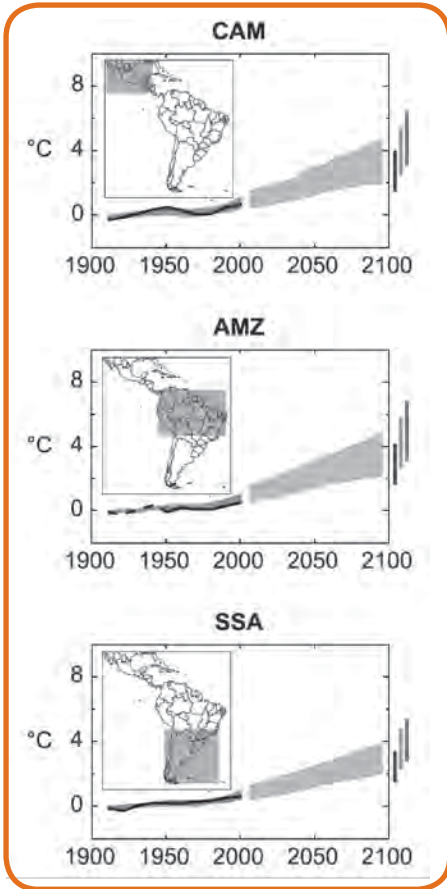
Figure 6. Multi-model projections of temperature increases for different regions of Latin America (gray envelope for the A1B emissions scenario). Bars at the right of the graph indicate the range of projected temperatures increases at the end of the century with lower (left) or higher (right) greenhouse gas emissions (Ch. 11, IPCC, 2007).
