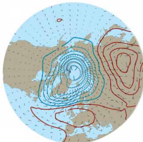
Summer Arctic Oscillation pattern
