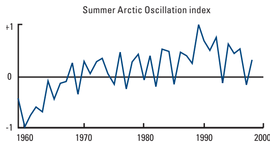
Summer Arctic Oscillation pattern
