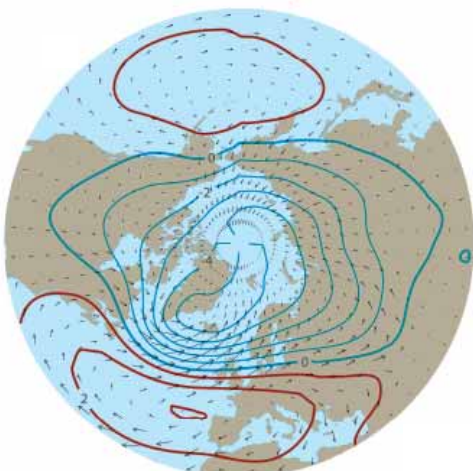
Winter Arctic Oscillation pattern
