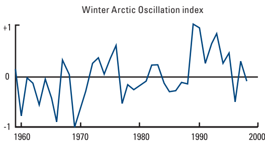
Winter Arctic Oscillation pattern
